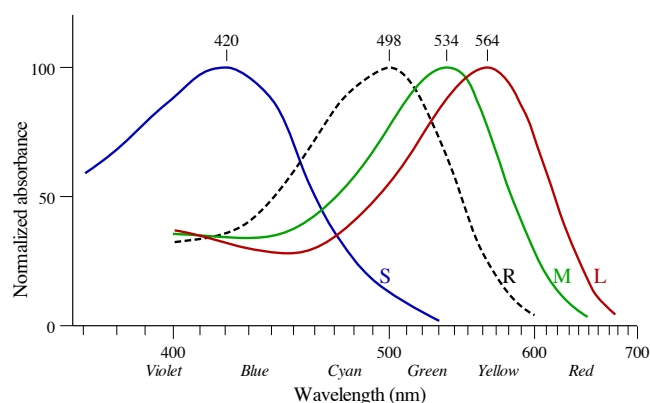
Figure 2: Normalized absorbance spectra of human cone cells, S, M, and L types and rod cells, R, cells responsible for black and white vision in dim lighting conditions [7].
