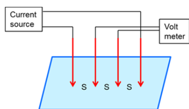
Figure 3. Principle of 4-point probe measurement for sheet resistance. S is needle spacing. The edges of the sample should be 4*S.
