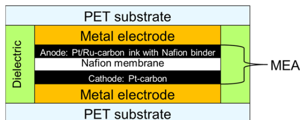
Figure 1. Layers for a printed 1-cell DMFC device.
