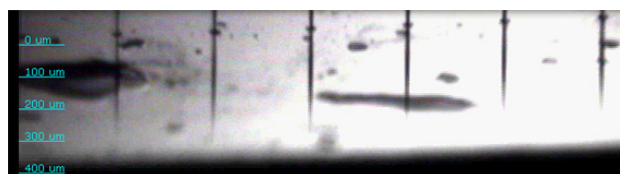
Figure 6. Drop formation of the water based ink with DMP-2831 printer.
