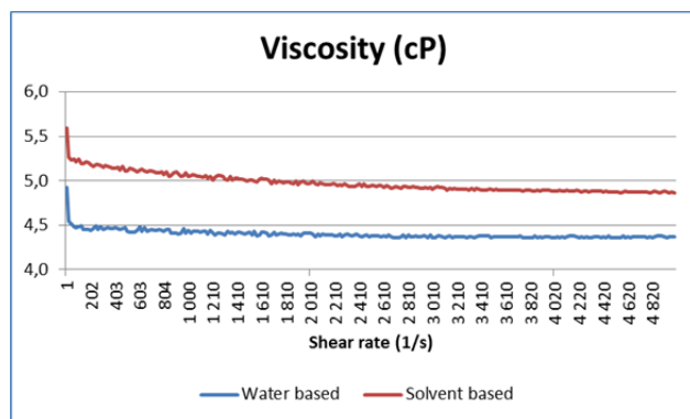
Figure 5. Viscosity curves for the water based and the solvent based inks.
