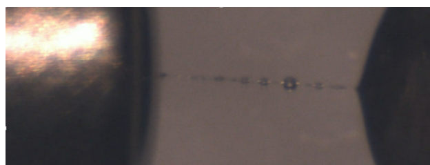
Figure 6. Polypropylene filament formation and droplet breakup behavior.
