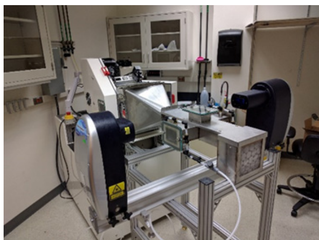
Figure 3. PARC's room temperature FEA test unit, including Malvern Spraytec particle sizer.
