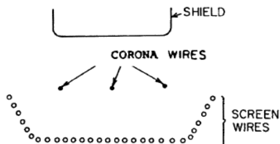
Figure 10. Basic layout of a scorotron charging device. [2]
