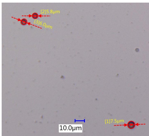
Figure 8. Sample particles of polypropylene sprayed onto a glass slide. Diameters represent diameters of impacted droplets, not diameters of in-flight droplets.
