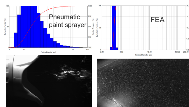
Figure 5. Comparison of drop sizes produced from FEA technology (right) and a pneumatic paint sprayer (left). FEA produces small, spherical, monodisperse droplets that are ideal for high resolution processing.
