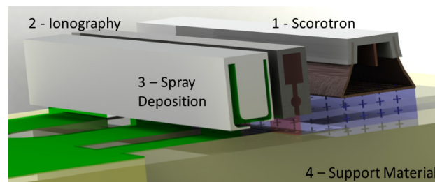
Figure 9. Digital patterning steps in PSD. (1) a scorotron is used to deposit a blanket charge, (2) the charge is selectively removed with an air assisted ionographic printhead, and (3) oppositely charged spray is deposited onto remaining charged areas. Following these steps, a (4) support material is filled into all remaining areas and (not shown) any remaining charge is neutralized.
