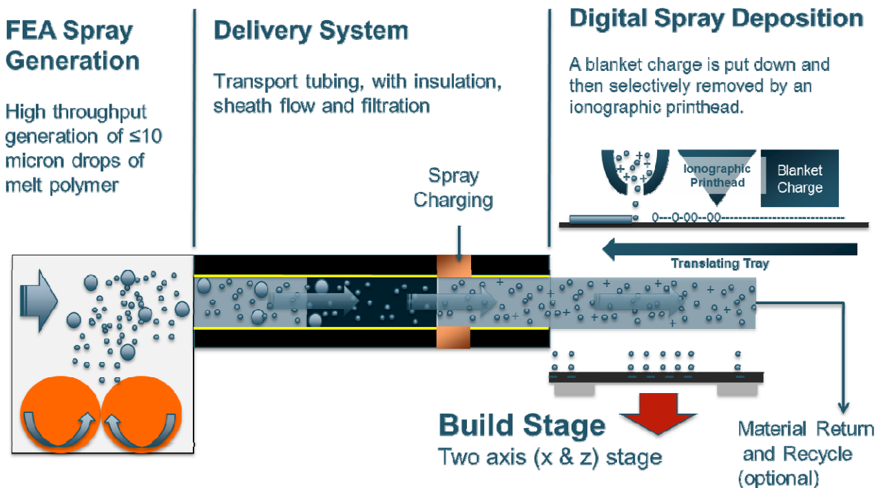
Figure 1. Polymer Spray Deposition process steps. From left to right, an aerosol is first produced using Filament Extension Atomization (FEA), it's then delivered to the target substrate and charged, the spray is then digital deposited onto the substrate. Digital patterning is achieved through blanket charging and then selective charge neutralization through ionographic printing.
