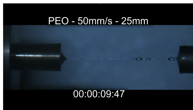
Figure 4. Filament breakup behavior of water, 0.2% polyethylene oxide, and 26% glycerol stretched between two pistons. The material can be observed forming filaments and forming small beads on a string.
