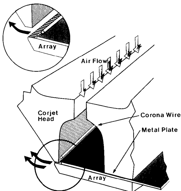
Figure 11. Cross section of a Corjet printhead, developed by the Xerox Corporation. [3]
