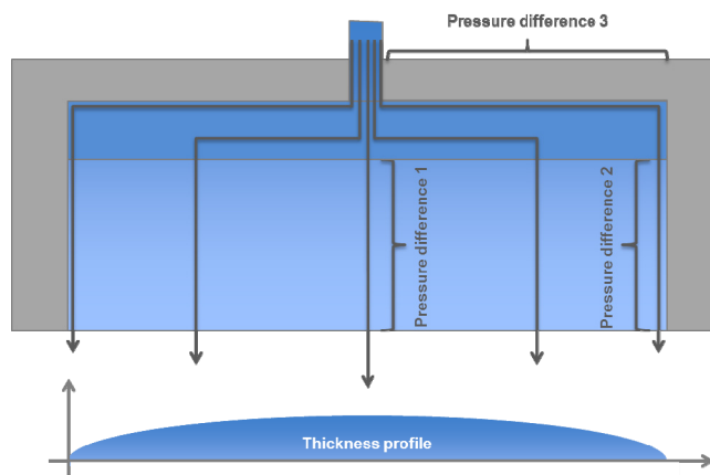
Figure 3 Theoretical thickness profile of a Slot Die
