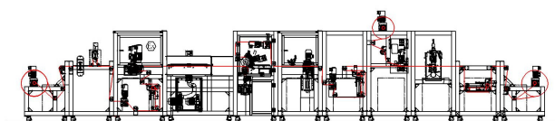
Figure 2 Drawing of a Coatema Coating machinery with nano-imprinting unit
