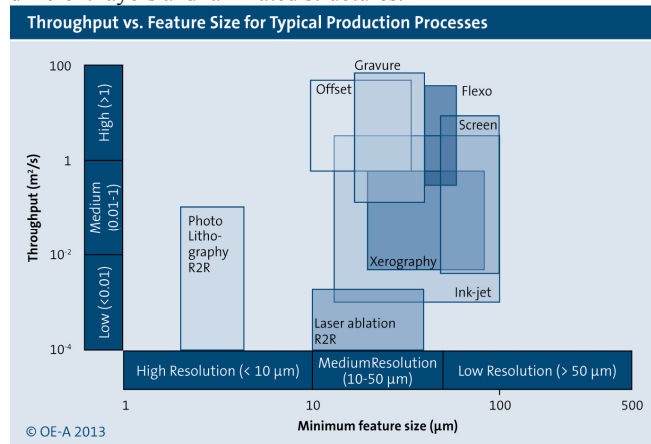
Figure 1 Throughput vs. Feature Size for Typical Production Processes
