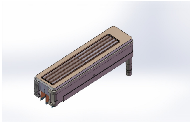
Figure 9 720 dpi printhead concept incorporating 4 edge-mounted actuators
