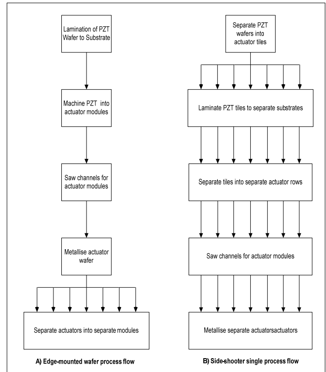
Figure 3 Comparison of edge-mounted and side-shooter actuator manufacturing process flows
