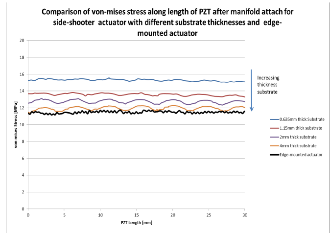
Figure 5 Comparison of stress distribution within PZT after manifold attach for central section of side-shooter and edge-mounted actuators
