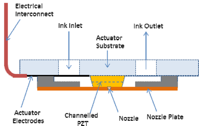
(a) ‘Side-Shooter’ Actuator
