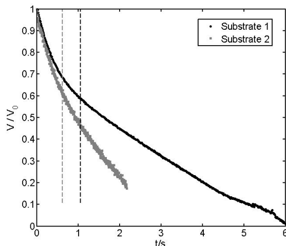
Figure 5. The evaporation rate of a 50%v ethanol/water droplet containing 0.1%v 1- \mu m polystyrene spheres on two coated substrates at a RH of 0.5. Substrate 1 has a higher initial contact angle than Substrate 2 (see Fig. 6). Vertical dashed lines indicate when R_{g,min} occurs on each substrate.
