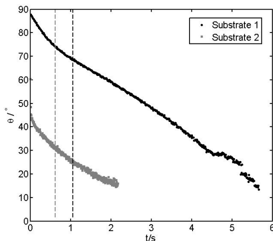
Figure 6. The contact angle evolution of a 50%v ethanol/water droplet containing 0.1%v 1- \mu m polystyrene spheres on Substrate 1 (high initial contact angle) and Substrate 2 (lower initial contact angle) at a RH of 0.5. Vertical dashed lines indicate when R_{g,min} occurs on each substrate.
