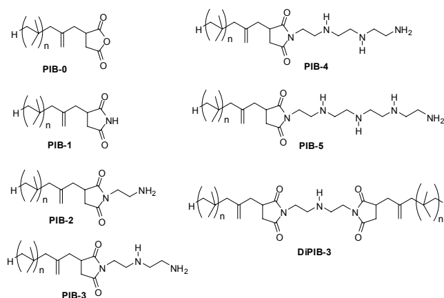
Figure 2. Surfactants studied
