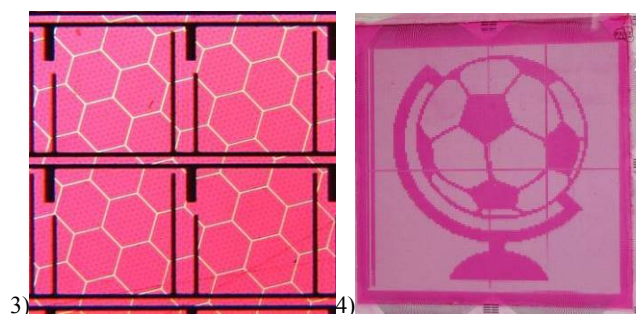
Figures 3. Transmission optical micrograph of integrated transparent TFT pixels with frontplane cells. 4) Integrated flexible frontplane with transparent oxide TFT backplane showing pixelation (16834 pixels).
