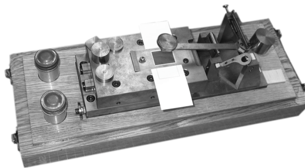
Figure 1: Spherical stylus scratch tester from ISO 18922
