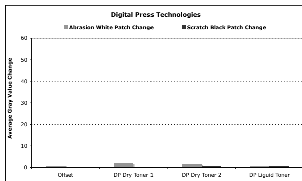
Figure 6: Comparison of white patch average gray value change caused by abrasion and black patch average gray value change caused by scratch damage for digital press technologies compared to a benchmark offset print.
