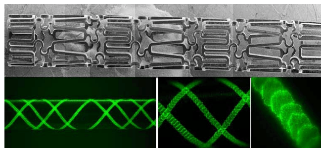
Figure 8 1.5mm coronary stent above, 100µm spots of anti-restenosis drug printed onto 1.5mm diameter polymer coated stent blank.
