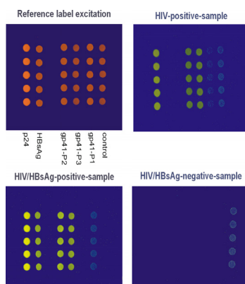
Figure 3 Immunoassay, ink-jet deposited spots ~100µm (courtesy Boehringer-Roche).
