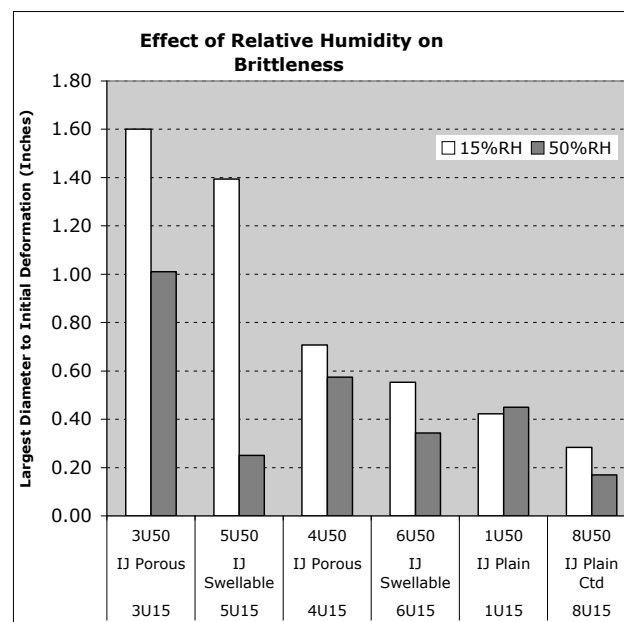
Figure 5: Largest Diameter to Initial Deformation (Inches) for Various Inkjet Papers 15% RH vs. 50% RH, Length Unprinted at 23°C
