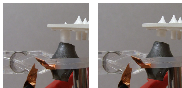
Figure 9. Balanced dual diaphragm actuator with pop-out spike in retracted and deployed positions.
