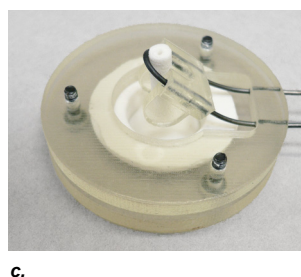
Figure 5. Nitinol lever-actuated spike (a) retracted, (b) deployed, and (c) underside view showing Nitinol lever arrangement with spike in its retracted position.
