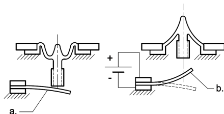
Figure 6. IPMC bending actuator mounted beneath a pop-out spike. The actuator in relaxed position (a) and actuated position (b).
