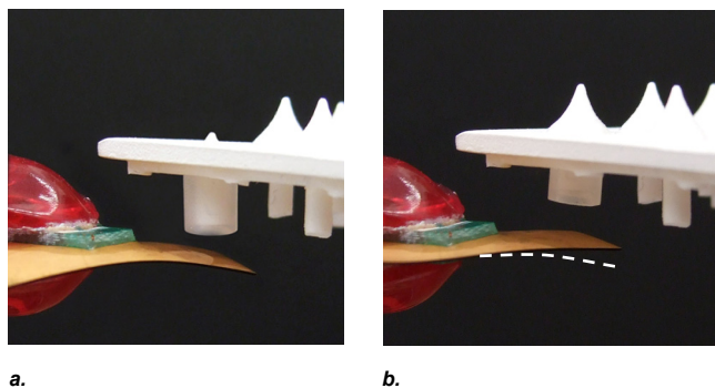
Figure 7. Pop-out spike with IPMC actuation (a) retracted, and (b) deployed, where the dashed line indicates the shape of the IPMC bending actuator in its previously relaxed position.
