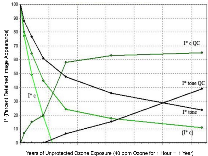
Figure 11. Ozone exposure to prints made with obsolete Canon ChromaPLUS inks and PR-101 porous photo paper printed with a Canon i9900 printer.
