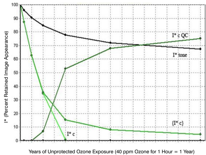
Figure 10. Unprotected ozone exposure of prints made with 3rd-party Calidad inks (from Australia) printed with an Epson C87 printer.
