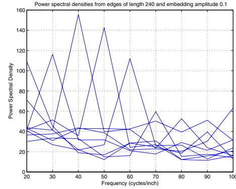
Figure 4. PSDs for each frequency embedded with amplitude 0.1
