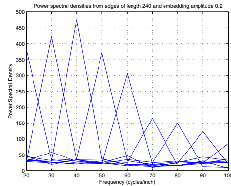
Figure 5. PSDs for each frequency embedded with amplitude 0.2
