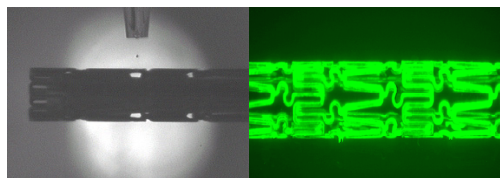
Figure 9. Left: the process of stent coating. Right: coated stent by ink-jet process.
