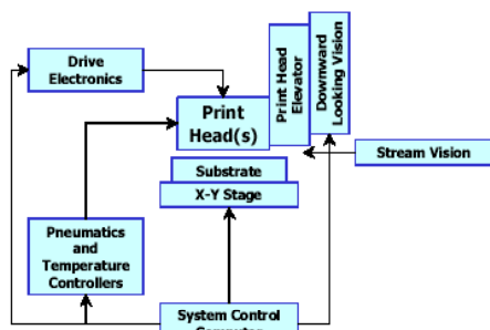
Figure 1. JetLab ® system block diagram.
