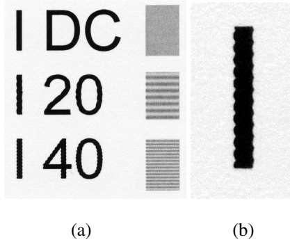
Figure 2. (a) Demonstration of exposure modulation in different images. (b) Magnified letter I in the third row of (a)
