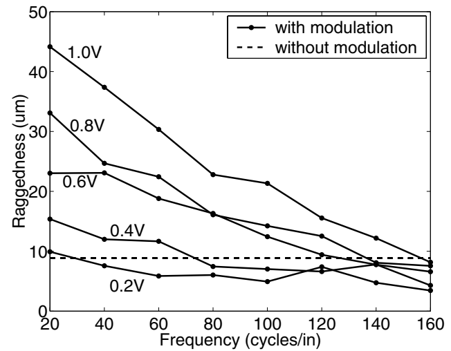
Figure 3. Relationship between exposure modulation with amplitude in 0.2~1.0 volts range and spatial frequency
