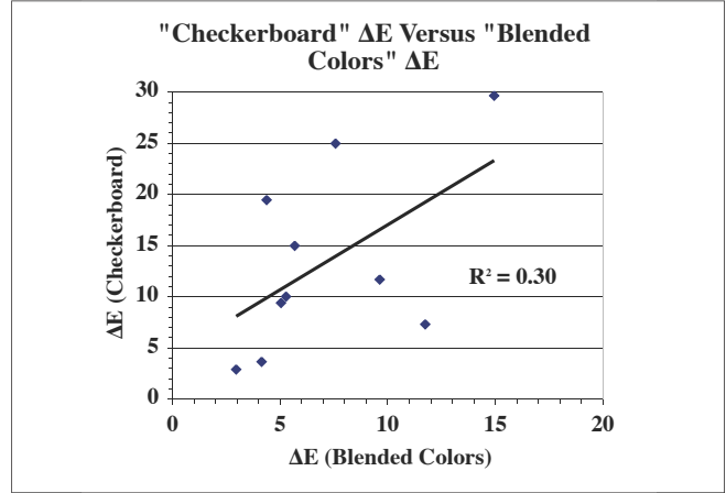
Figure 10. Ten print systems correlated using worst 10% ΔE averaged data criterion.
