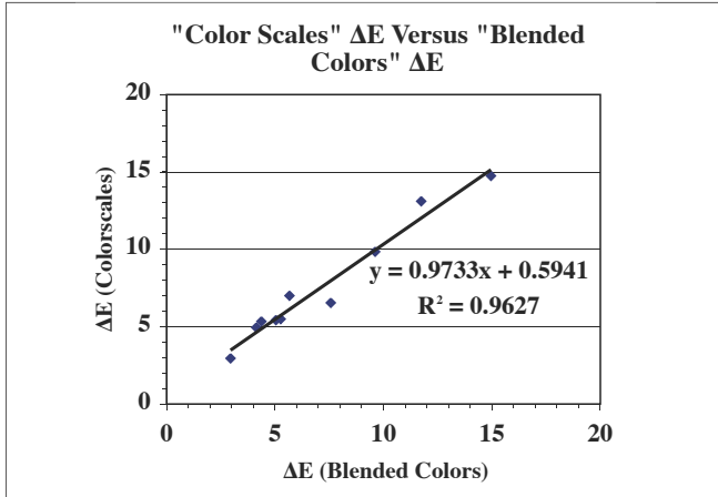
Figure 9. Ten print systems correlated using worst 10% ΔE averaged data criterion.
