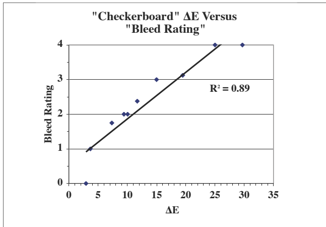
Figure 11. Ten print systems correlated using worst 10% ΔE averaged data criterion.
