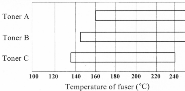
Figure 1. Fusing ability of Toner A and Toner B
