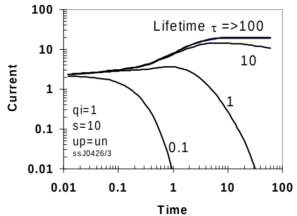
Figure 3. Current vs. time for samples with different lifetime to deep trapping \tau .
