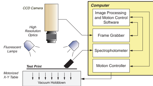
Figure 1. Schematic representation of QEA's IAS-1000 Automated Image Analysis System
