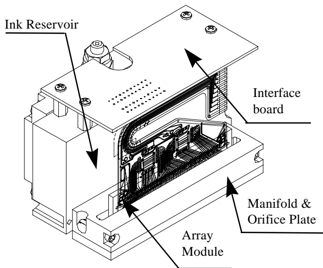
Figure 1. Spectra's 128 jets, 600dpi CCP Printhead.
