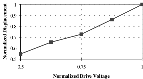
Figure 4. PZT displacement as a function of drive voltage
