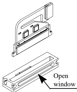
Figure 2. Modified manifold assembly with an opening on collar for the measurement of transducer's surface.
