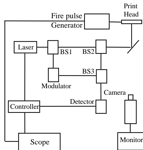
Figure 3. A schematic of the laser Doppler vibrometer measuring system.
