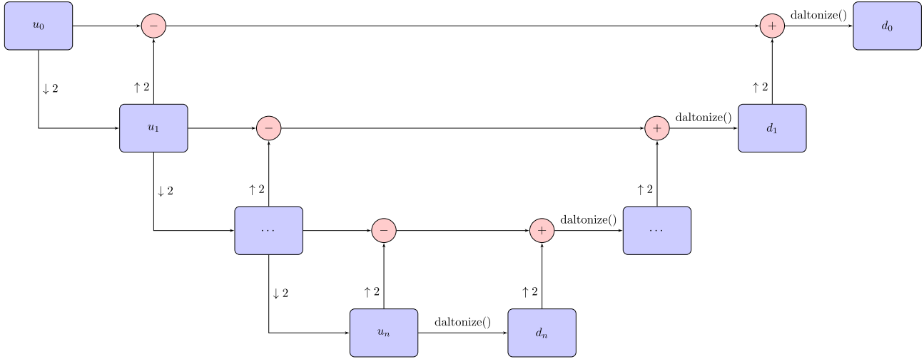
Figure 2. Multiscaling pyramid structure, where “ \downarrow 2 ” indicates minimizing the image to half its size, “ \uparrow 2 ” indicates enlarging it to double its size, and “daltonize()” indicates the daltonization step at each iteration.
