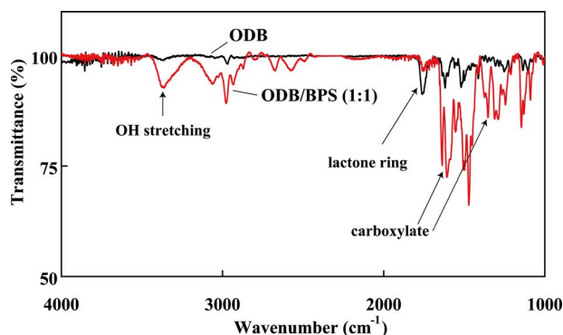
Figure 8. Infrared spectra of spin-coated ODB alone and ODB/BPS (=1:1).
