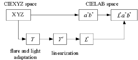
Figure 4. Procedure for lightness enhancement using the lightness adaptation model.
