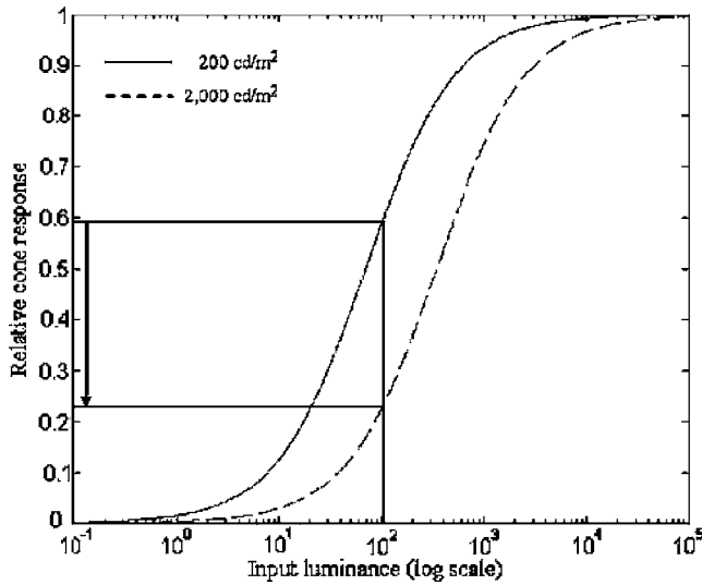
Figure 3. Cone response curve according to the intensity of the ambient light.
