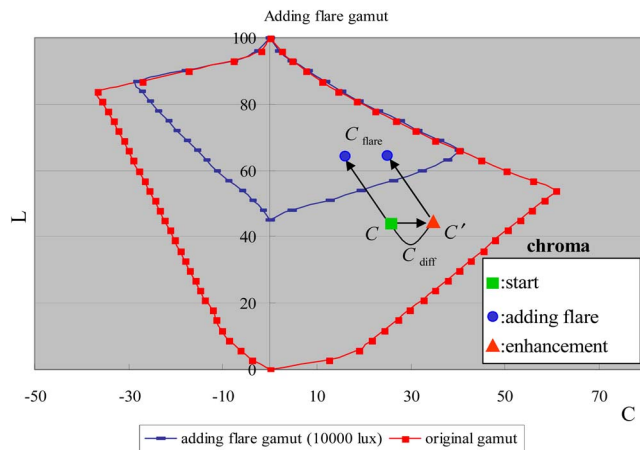
Figure 7. Concept of chroma compensation based on chroma difference.
