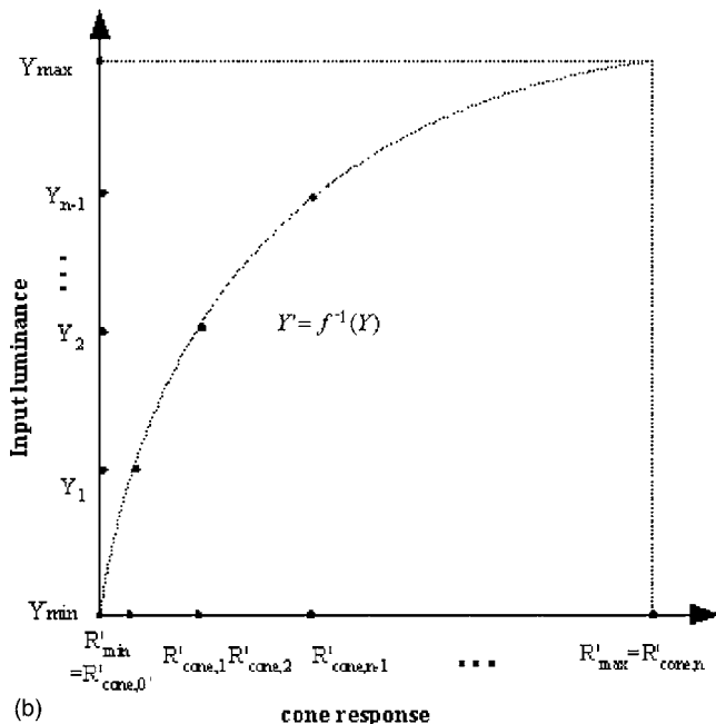
Figure 5. Linearization method: (a) construction of the cone response curve using piecewise linear interpolation and (b) construction of the linearized cone response curve using piecewise linear interpolation.
