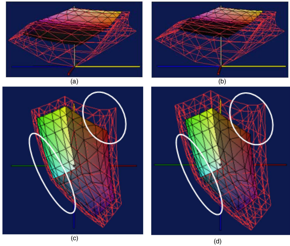
Figure 2. Comparison of the gamut under an outdoor environment (solid frame) and an indoor environment (wire frame): (a) 5000 lux (side), (b) 10 000 lux (side), (c) 5000 lux (top), and (d) 10 000 lux (top).
