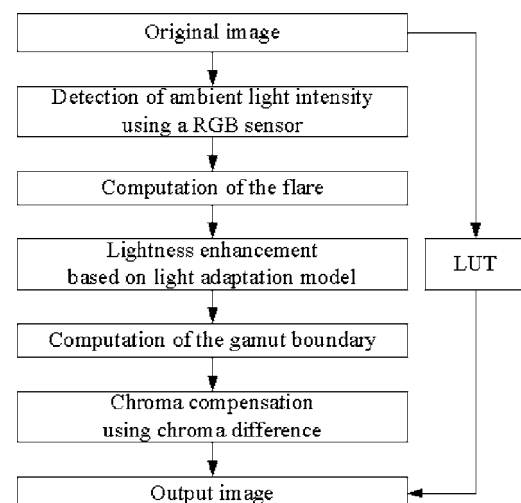
Figure 1. Flowchart for the proposed algorithm.
