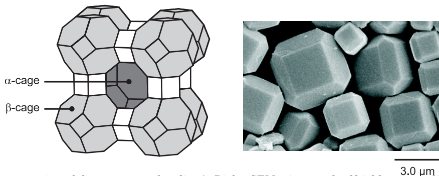
Figure 10. Left: Representation of the structure of zeolite A. Right: SEM micrograph of highly pure sodium zeolite A (prepared according to reference 60) used for the synthesis of quantum-sized silver sulfide clusters.
