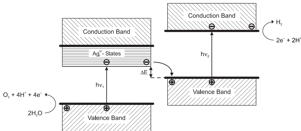
Figure 14. Qualitative scheme of a tandem device based on a Ag/AgCl photoanode and an appropriate semiconductor as photocathode.
