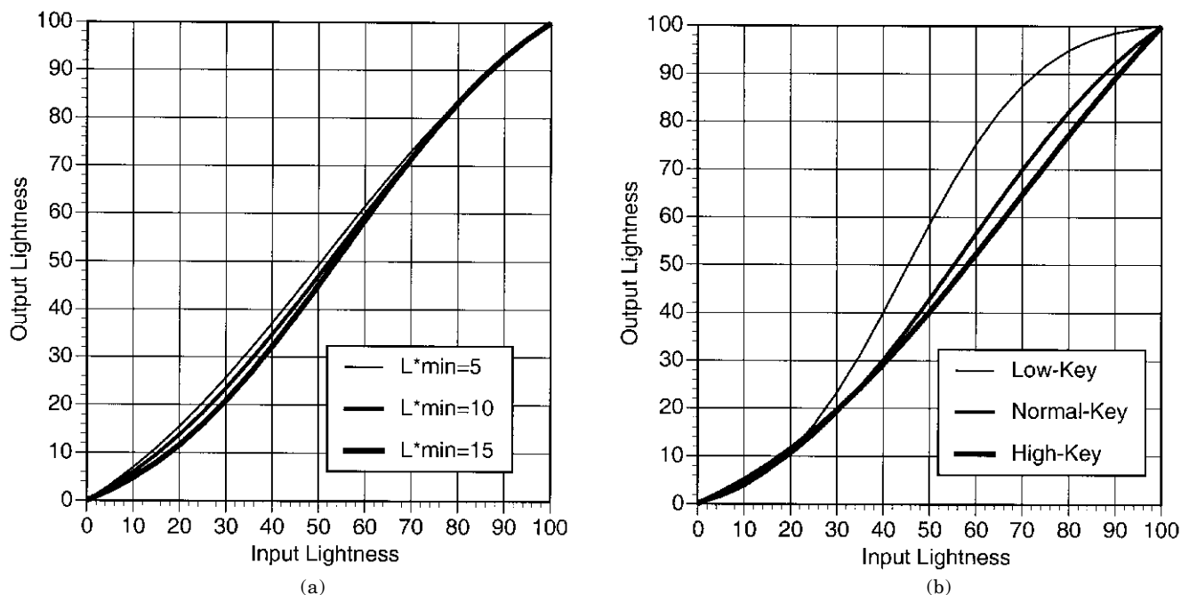
Figure 4. Sigmoidal remapping functions used to maintain perceived lightness contrast for (a) different output dynamic ranges and (b) different image content. (Note: The curves have been normalized to a range of [0-100] to illustrate the differences in contrast and curvature.)
