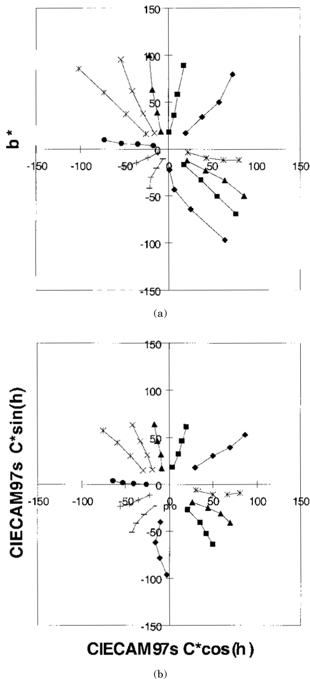
Figure 2. Hung and Berns 12 lines of constant perceived hue plotted in (a) CIELAB and (b) CIECAM97s.
