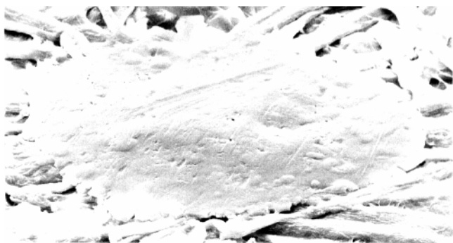
Figure 32. A SEM of a fused phase-change ink drop on a paper that results from a offset drum transfer process.
