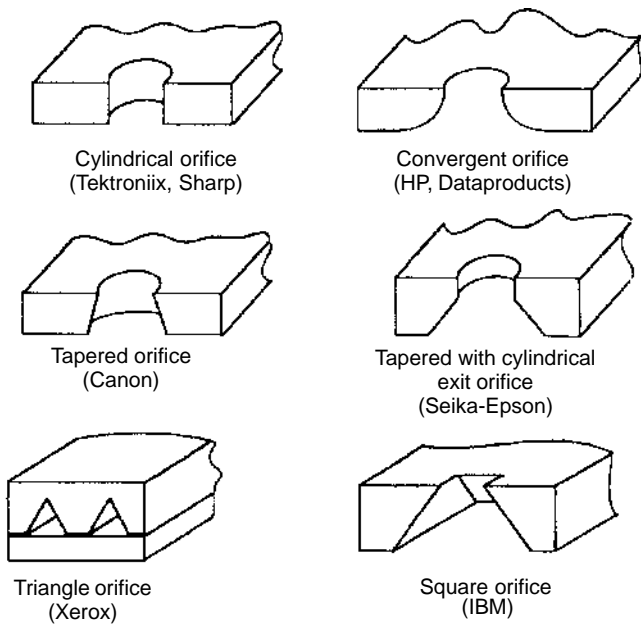
Figure 22. Various types of ink-jet printhead nozzle designs.
