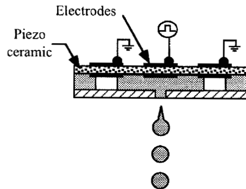
Figure 9. A shear-mode piezoelectric ink-jet design.
