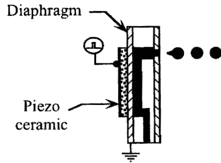
Figure 7. A bend-mode piezoelectric ink-jet design.
