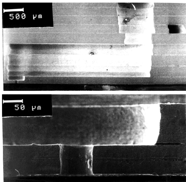
Figure 16. Cross section SEM photographs of a Tektronix stainless steel jet stack.
