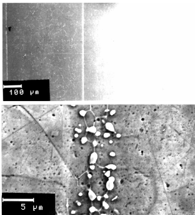
Figure 17. Cross section SEM photographs of a bond line in a Sharp stainless steel jet pack.
