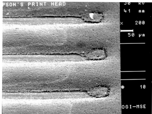
Figure 21. A SEM photograph of the thick film PZT on the zirconia diaphragm in the Epson Color Stylus 800 printhead.
