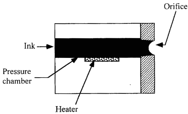
Figure 5. A side-shooter thermal ink-jet.
