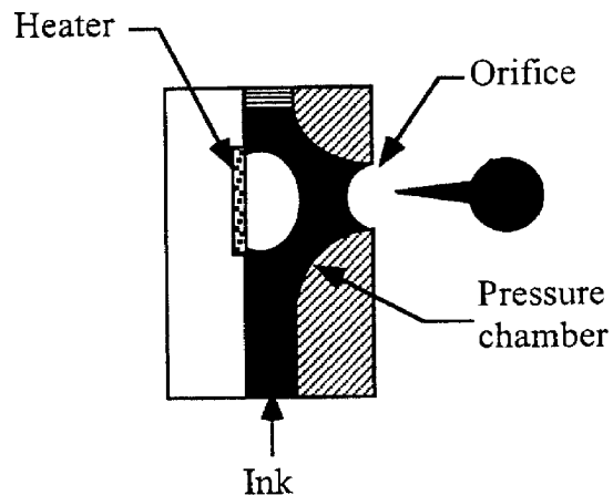
Figure 4. A roof-shooter thermal ink-jet.
