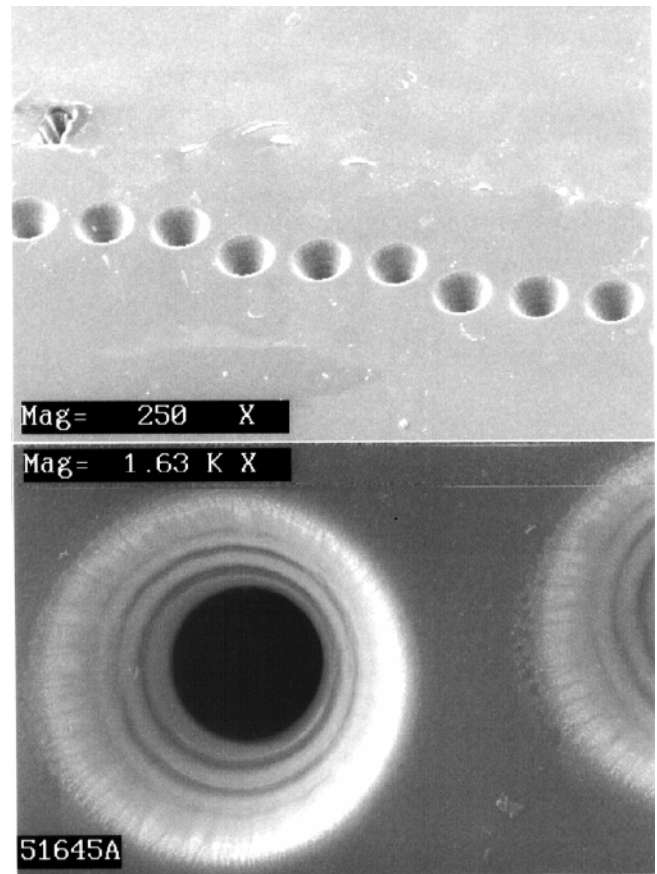
Figure 24. SEM photographs from the entrance side of a laser ablation polyimide nozzle plate.
