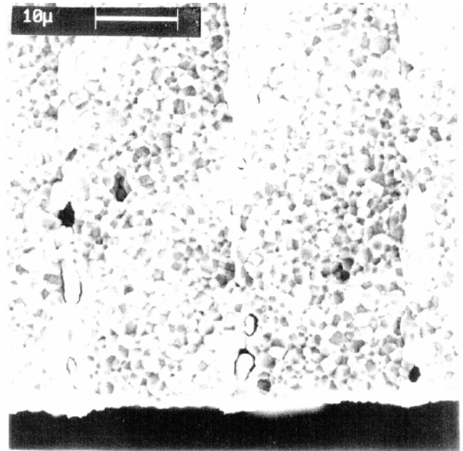
Figure 20. A SEM photograph of a multilayer piezoceramic driver in the Epson Stylus 800 printhead.
