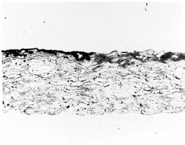
Figure 34. A cross section light microscope of pigment-based (on the left) and dye-based (on the right) inks on paper.
