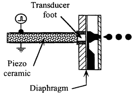
Figure 8. A push-mode piezoelectric ink-jet design.
