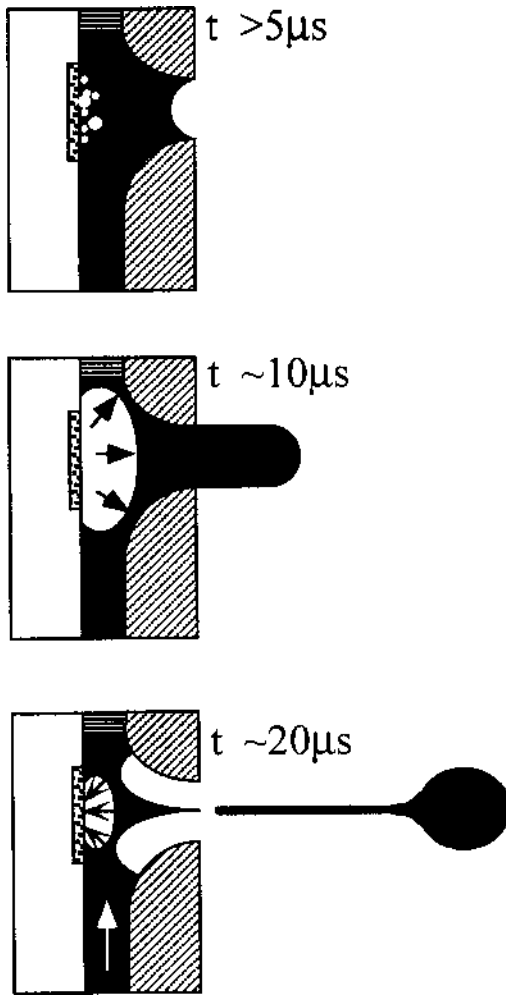
Figure 10. Drop formation process of a thermal ink-jet.
