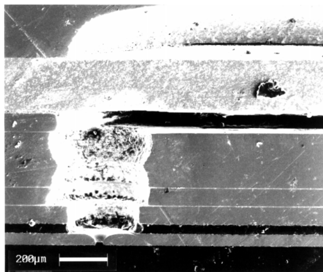
Figure 18. A cross section SEM photograph of a Spectra printhead.
