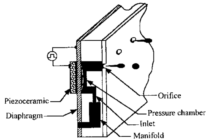
Figure 14. The basic configuration of a piezoelectric printhead.
