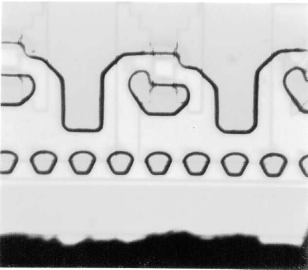
Figure 13. A light microscopic photograph of a channel in the Hewlett-Packard DeskJet 890C color printhead.
