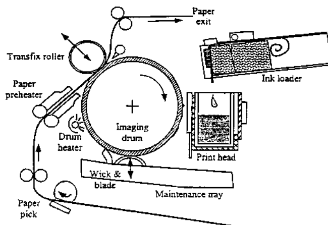
Figure 30. The basic configuration of the Tektronix's Phaser 350 offset drum transfer ink-jet printer.
