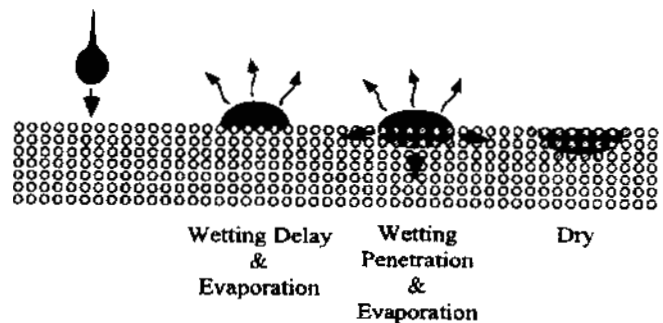
Figure 27. Drying mechanisms of a water-based ink-jet drop on a plain paper.
