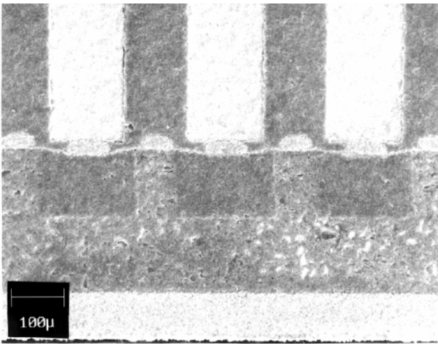
Figure 19. A cross section SEM photograph of an Epson Stylus 800 printhead.
