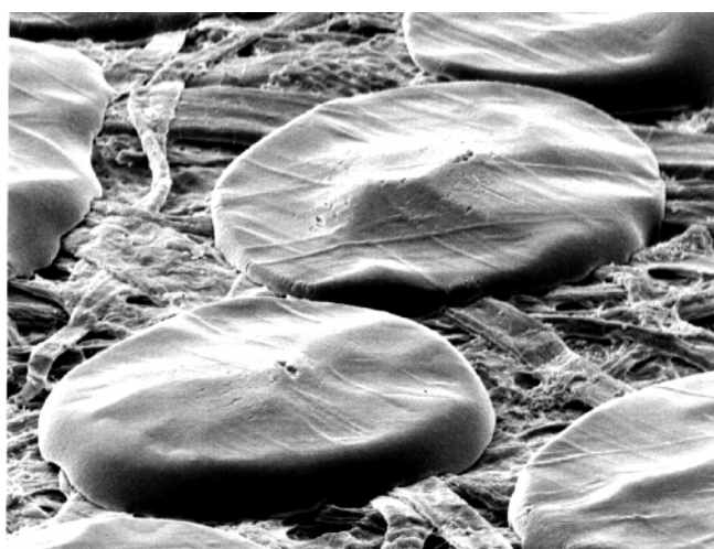
Figure 29. A SEM photograph of phase-change ink drops after fuse by cold pressure rollers.
