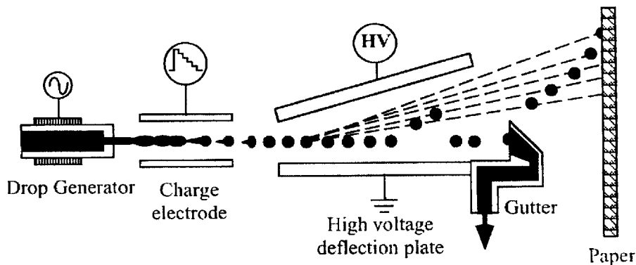
Figure 3. Continuous ink-jet: A multiple-deflection system.
