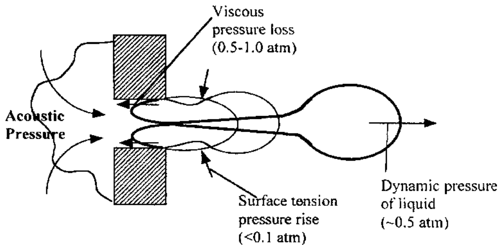
Figure 15. The basic pressure requirement for ejecting an ink droplet.
