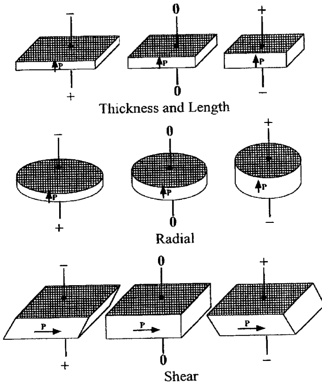
Figure 6. Basic deformation modes of a piezoceramic plate.
