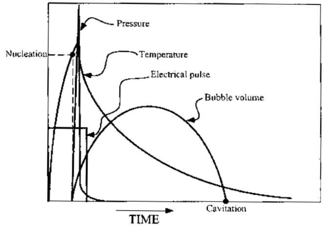
Figure 11. Pressure, temperature, and bubble volume changes during a drop formation cycle of thermal ink-jet.
