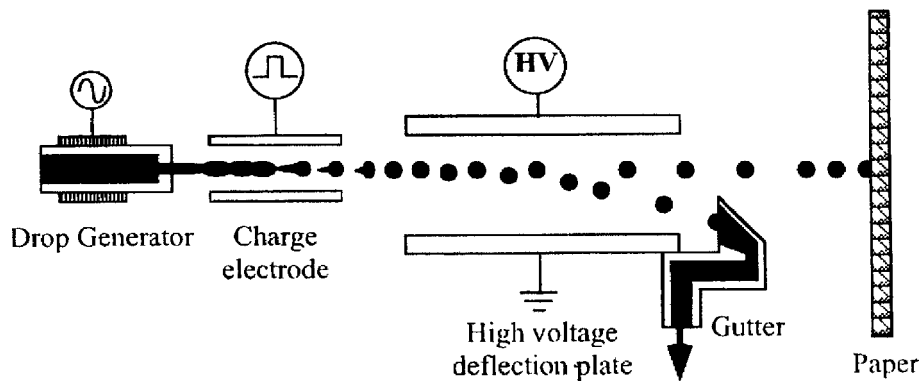
Figure 2. Continuous ink-jet: A binary-deflection system.
