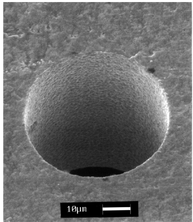
Figure 25. A SEM photograph of an EDM stainless steel nozzle.
