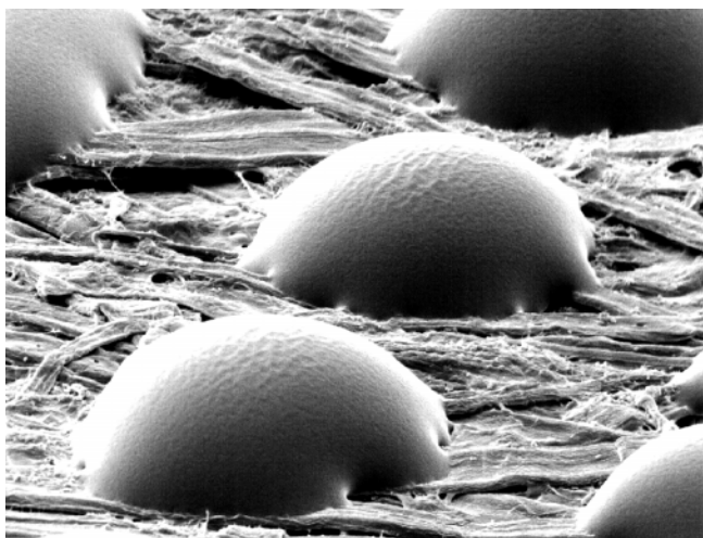
Figure 28. A SEM photograph of phase-change ink drops on the surface of a bond paper.
