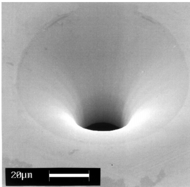
Figure 23. A SEM photograph from the entrance side of an electroformed Ni nozzle.
