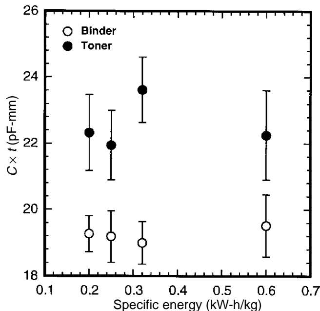
Figure 9. Polarizability of the binder and the toner samples at room temperature; measurement frequency: 1 kHz.
