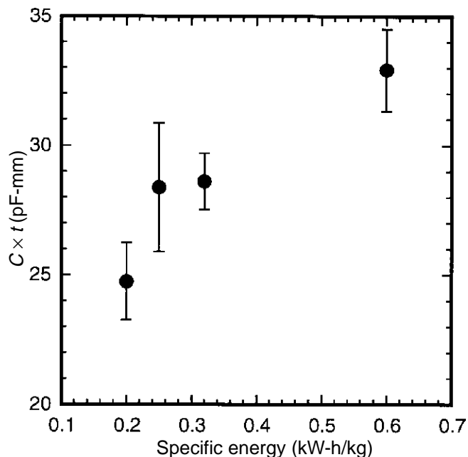
Figure 10. Polarizability of the toner samples at 150°C; measurement frequency: 1 kHz.
