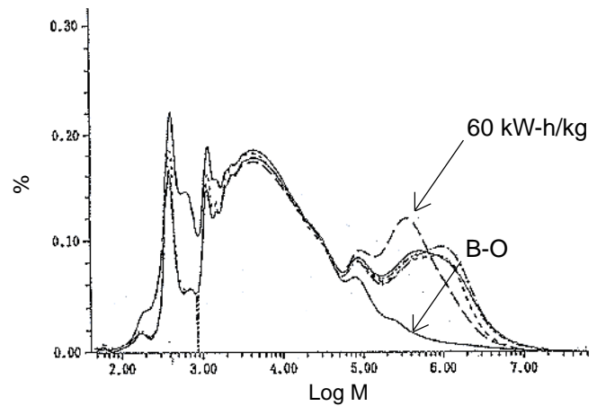
Figure 7. Molecular weight distribution of the binder samples; B-O is the unprocessed binder for comparison.
