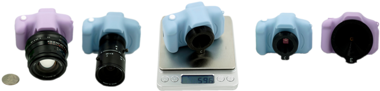
Figure 4. A US quarter and Kentucky's Adorable Micro Format (KAMF); blue is visible light C mount, purple is full-spectrum E/FE mount
