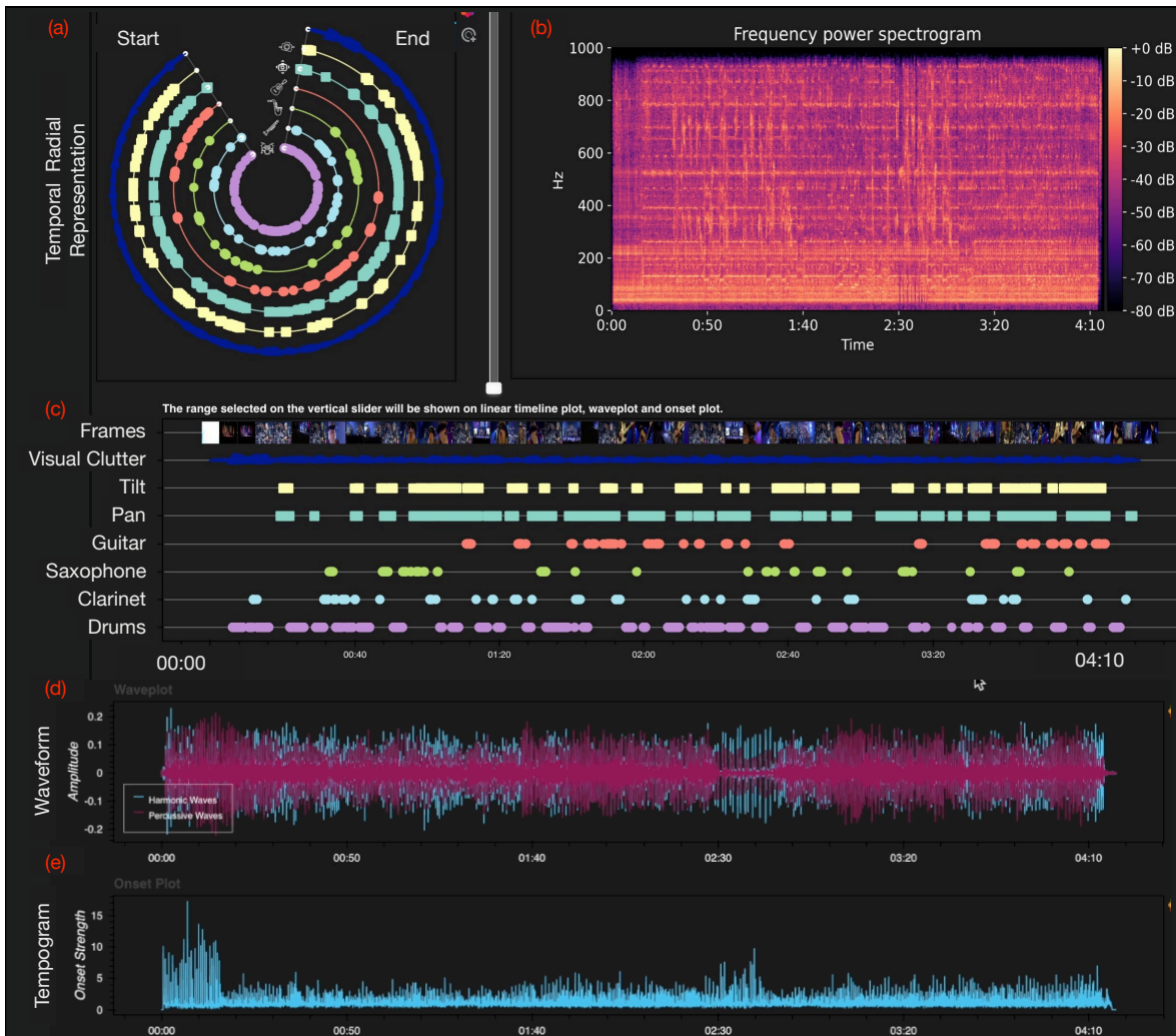
Figure 1. Screenshot of our solution. (a) presents a radial overview of the temporal distribution of audiovisual features for a selected song, (b) shows the power spectrogram view of the song, and below shows the timeline view displaying the (c) discrete and (d,e) continuous audiovisual features over time.
