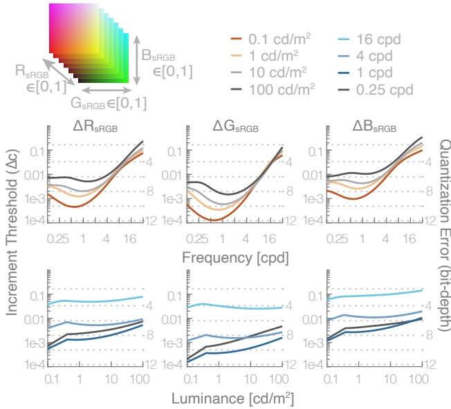
Figure 2: sRGB using ITU-R BT.709 color primaries [20]. Top row: CTF with respect to frequency. Bottom row: CTF with respect to luminance. Left y-axis: increment thresholds. Right y-axis: quantization error. Dotted grey lines indicate quantization error for different bit-depths. All CTF figures (Figs. 2–9) follow the same formatting convention.
