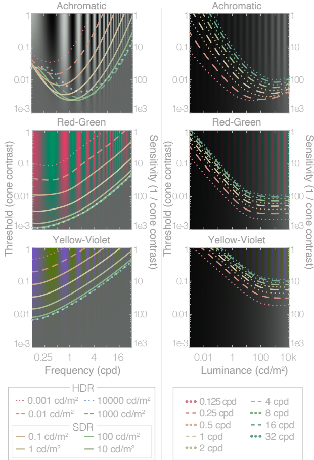
Figure 1: Spatio-chromatic contrast threshold functions (CSFs) along the cardinal directions of the DKL color space [12, 13]. Left column: CSFs as a function of frequency. Right column: CSFs as a function of luminance. Left y-axis: Contrast threshold. Right y-axis: Contrast sensitivity.
