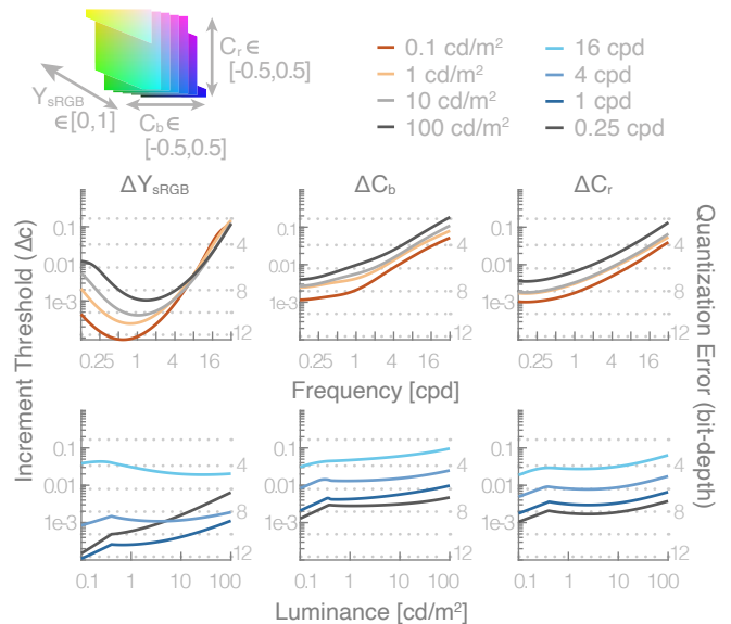
Figure 5: YC_bC_r using ITU-R BT.709 color primaries [20].
