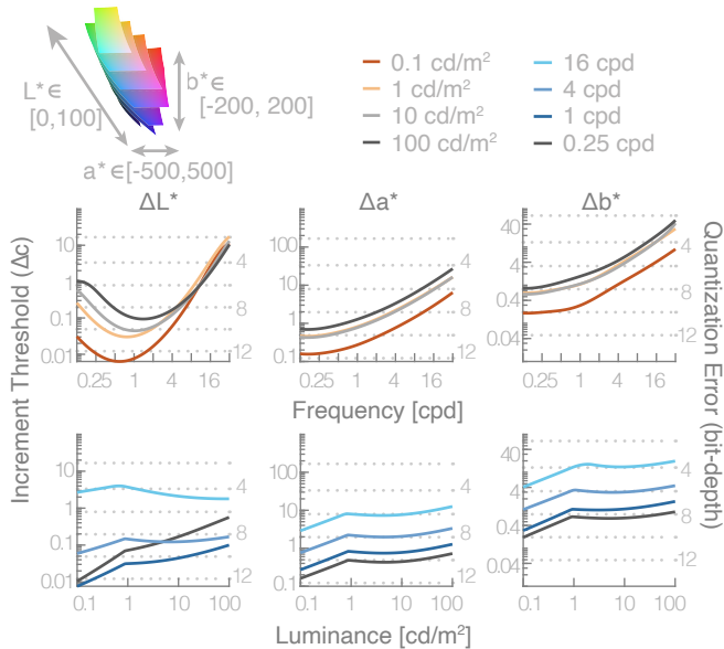
Figure 8: CIE L^*a^*b^* using ITU-R BT.709 color primaries [20].
