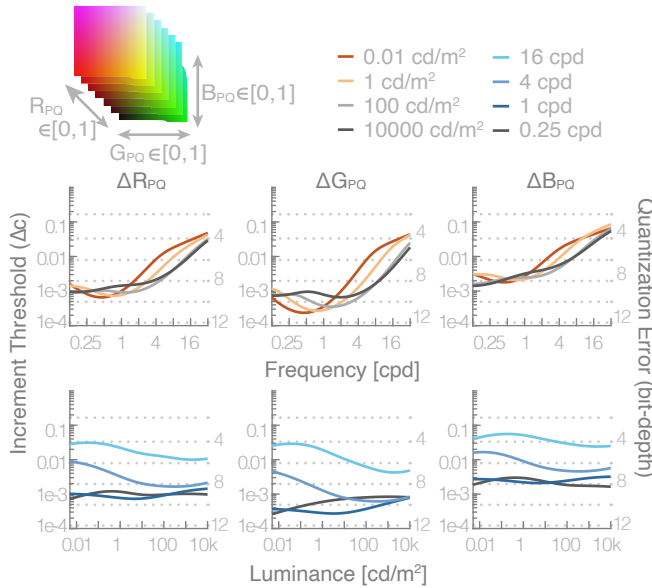
Figure 3: PQ-RGB using ITU-R BT.2020 color primaries [21].
