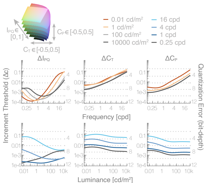
Figure 9: IC_T C_P using ITU-R BT.2020 color primaries [21].
