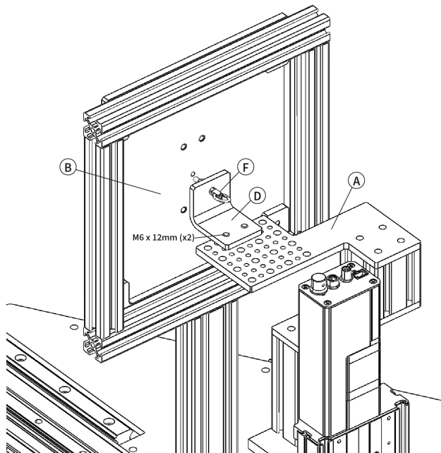
Figure 12. Retractable Spring Plunger Configuration for Camera X & Y axis Calibration
