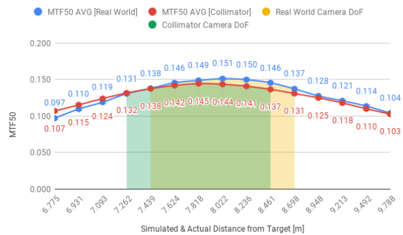
Figure 8. MTF50 VS Simulated/Actual Distance (8m Nominal)
