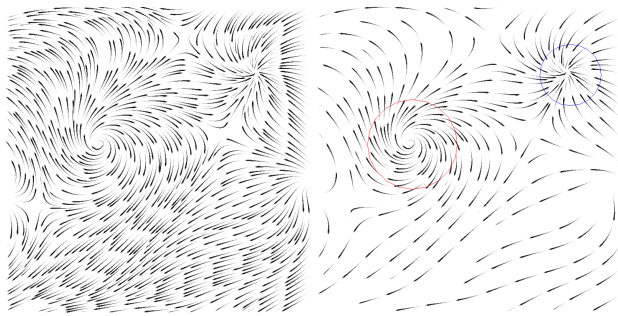
Figure 9. Our streamlines with directional cues (left) and directed streamlines with foveated rendering (right) that eliminates visual clutter.
