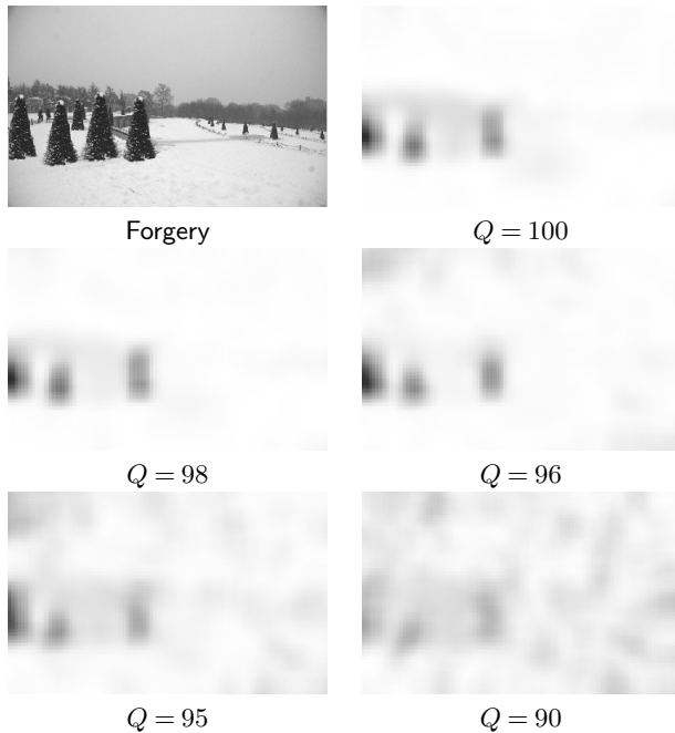
Figure 8. Output masks after compressing the forged image with quality factor Q . The added trees (upper left) were downscaled by 5%.
