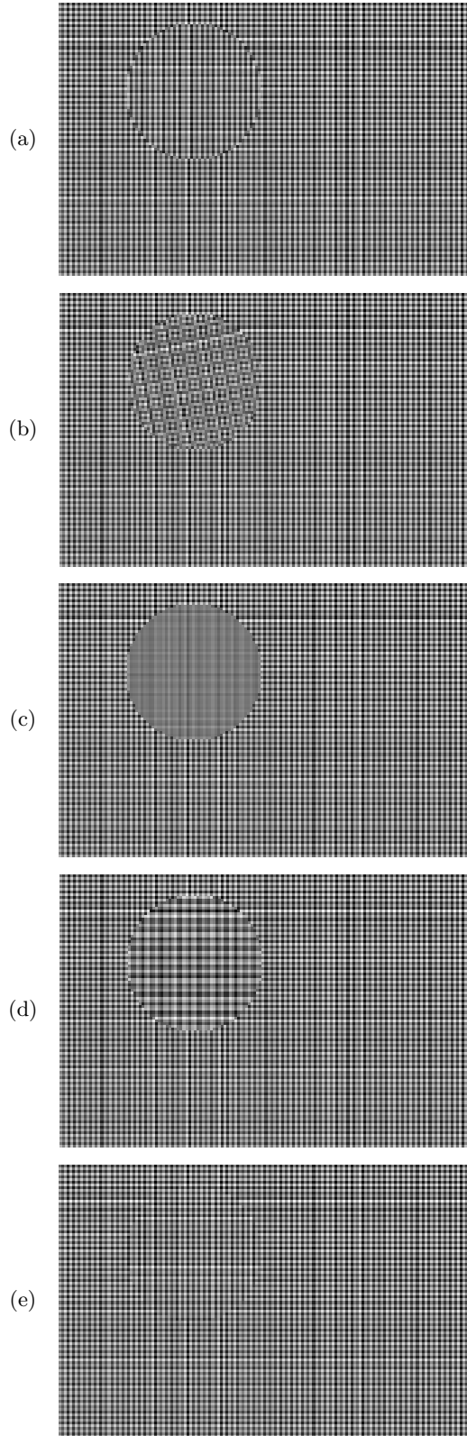
Figure 3. The effect of a circular area modification on the LP from image (a) in Figure 2: a) copy-paste shifted by an odd number of pixels, b) rotation, c) downsampling, d) upsampling, e) copy-paste shifted by an even number of columns.
