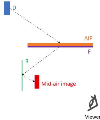
Figure 20 Proposed optical system that allows vertical mid-air images to be seen when viewers face upward.
