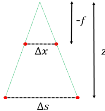
Figure 3. Light field EPI data generation
