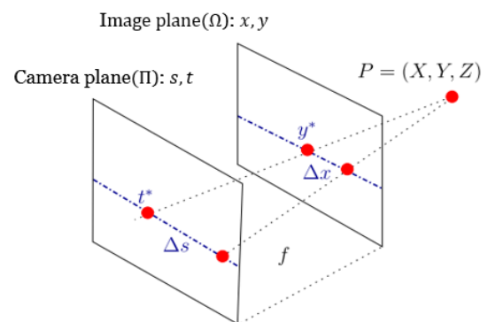
Figure 1. Light field camera plane structure
