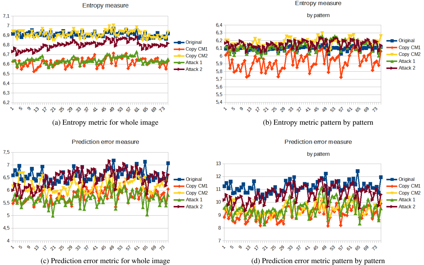
Figure 3: The metric values for original, copied and attacked samples using: a) Entropy metric for whole image, b) Entropy metric for every pattern, c) Prediction error metric for whole image and d) Prediction error for every pattern.
