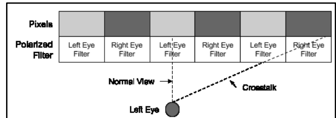
Figure 8. Off-axis crosstalk.
