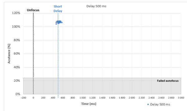
Figure 10. Device B - Autofocus performances at 1000 lux with proposed measurement
