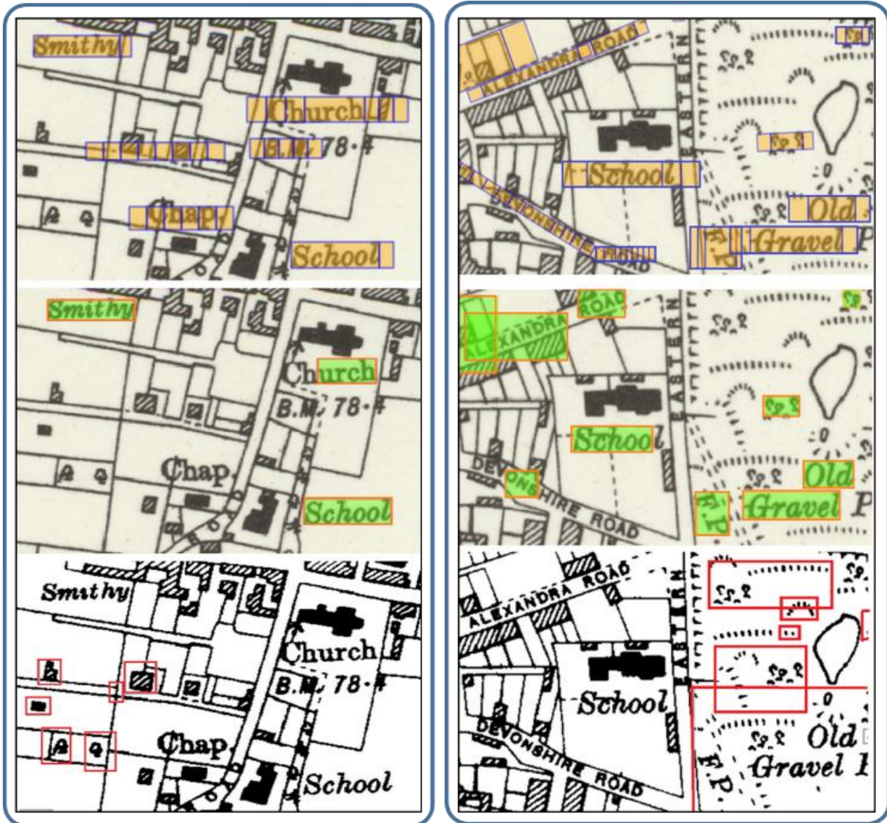
Figure 22. Example text detection results. The top images are the result of text detection from Strabo after using OTD. The middle images show the results of Strabo before using OTD. The bottom images show the results from Cao et al.'s algorithm.
