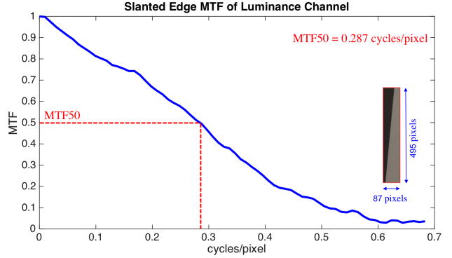
Figure 1: MTF measured on an iPhone 5 by slant edge analysis tool with (ISO 16067) Q-62 target. The cropped image on the right shows the vertical slanted edge being used.
