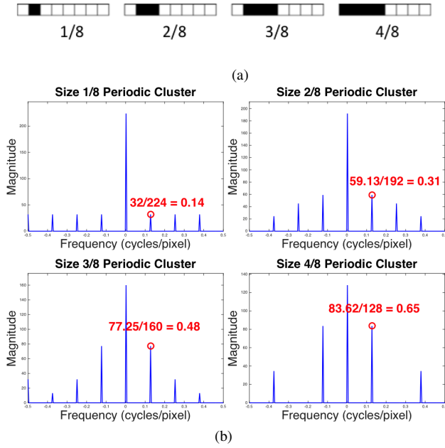
Figure 2: Relationship between peak spectral magnitude and 1D cluster width. (a) Cluster sizes 1 to 4. From left to right are non-periodic clusters with width 1/8, 2/8, 3/8, 4/8. (b) The DFTs of the corresponding periodic patterns.
