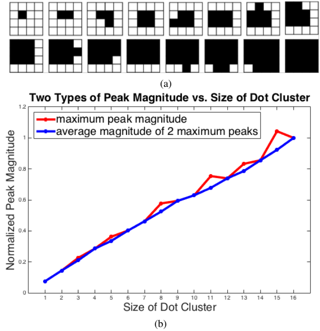
Figure 3: Relationship between peak 2-D DSFT spectral magnitude and 2D cluster area. (a) 2D highlight cluster sizes 1 to 16. The shape of the cluster is defined by [3]. Row one shows dot cluster sizes 1 to 8. Row two shows dot cluster sizes 9 to 16 (left to right). (b) Peak magnitude versus size of dot cluster. We use the highlight clusters defined in (a). The red line shows the maximum peak magnitude for the frequencies -0.5 < \mu < 0.5 , 0 < \nu < 0.5 . The blue line shows the normalized average peak magnitude of the two maximum peaks for the frequencies -0.5 < \mu < 0.5 , 0 < \nu < 0.5 .
