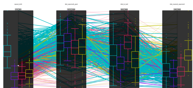
Figure 7: Box plots denoting density and statistical information for each cluster in each dimension. Statistically significant differences can be easily detected by comparing the boxes of the box plots.
