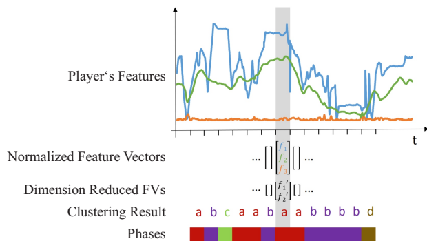
Figure 3: Feature-based approach to detect similar activity phases of a single player. Reprinted from [10].
