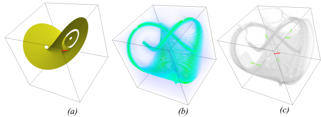
Figure 12: A stream surface placement of Lorenz flow based on |\nabla\Phi| field (a). (b) and (c) are the visualization of \Phi and |\nabla\Phi| field, respectively. The seeding curve of the stream surface is highlighted with red color.
