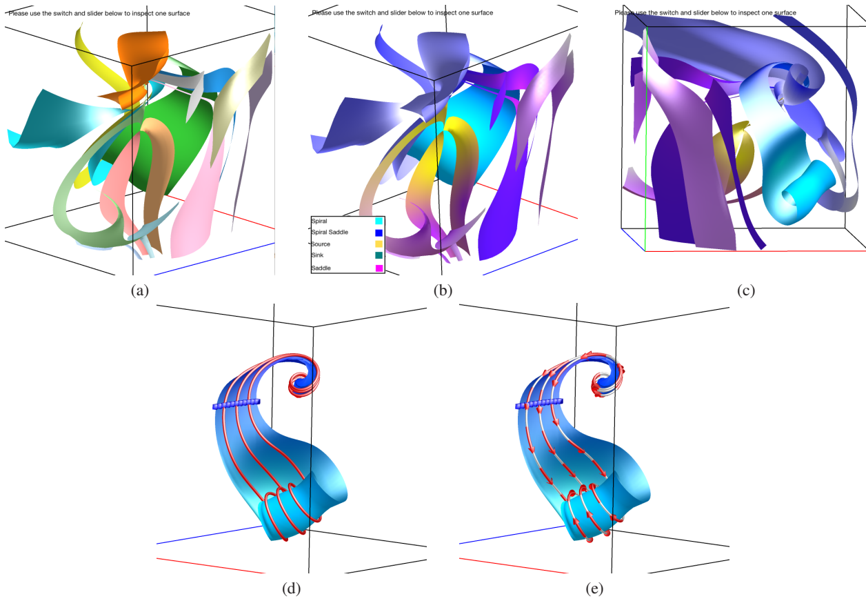
Figure 3. Stream Surfaces. (a) multiple surface overview with unique color for each surface, (b)-(c) multiple surface overview with coloring based on the types of related critical points, (d) single surface with streamlines, and (e) single surface with streamline animation.
