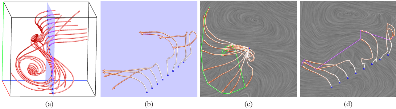
Figure 2. Field-lines. (a) streamlines, (b) pathlines, (c) pathline-streakline with LIC, and (d) pathline-timeline with LIC.
