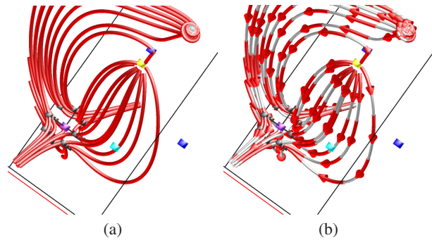
Figure 5. Streamlines around critical points via template-based seeding. (a) static streamlines and (b) dynamic streamlines with animated arrows.
