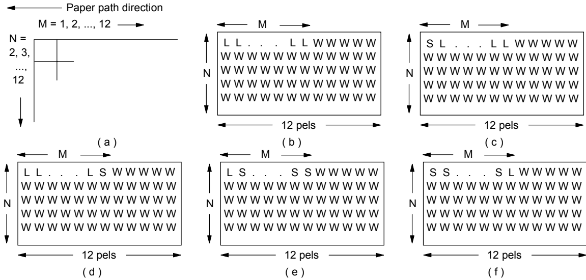
Figure 1. Experiments to determine consistent intermediate level print quality. a) For each level L ( L=1, 2, \dots, 15 ) and color ( C, M, Y, K ) print a 6 inch \times 5.5 inch grid of 1/2 inch square patches filled with N \times 12 cells containing a 1 \times M mark in a white background. b) Cell with mark at level L . c) Cell with leading pel saturated ( S=15 ). d) Cell with trailing pel saturated. e) Cell with non-saturated leading pel. f) Cell with non-saturated trailing pel.
