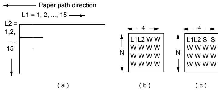
Figure 2. Additional experiments to determine consistent intermediate level print quality. a) For each color ( C, M, Y, and K ) print a 7.5 \times 7.5 inch grid of 1/2 inch square patches filled with 4 \times 4 cells. b) Cell with L1 and L2 pair of pels in a white background. c) Cell with L1 and L2 pair of pels followed by two saturated pels to make a line every fourth row in a white background.
