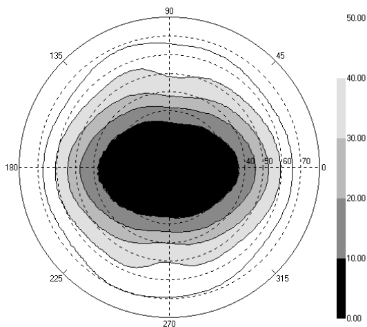
Figure 2. Isocontour polar plot of \Delta E^* for the white state of a typical MVA mode panel.
