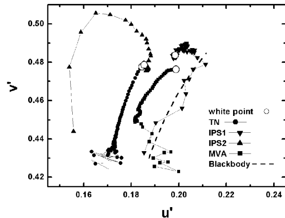
Figure 5. Typical chromaticity shift of grays.
