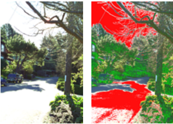
Figure 4. The left image (a) shows a PhotoYCC encoding of a color photograph tone-mapped with a linear operator. The right image (b) shows the out-of-gamut regions. Red areas are too bright or too dim, and green areas have inaccurate color.
