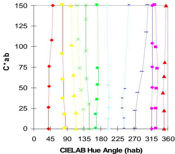
Figure 5. Twelve gridlines generated from the Hung and Berns data set. These gridlines are used to populate the 2D LUT.
