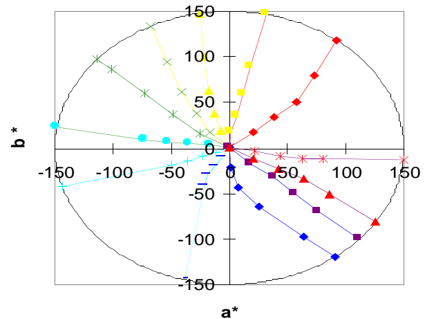
Figure 3. Extrapolation of Hung and Berns data out to C_{ab}^* = 150 .
