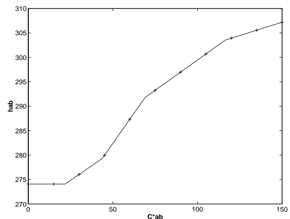
Figure 4. Example gridline calculation for the constant hue line at base-hue angle = 274.1 degrees. The figure shows that as the chroma increases along this hue line that the CIELAB hue angle increases. By linear interpolation between the Hung and Berns points it is possible to estimate the departure of hue (+), from the base-hue angle, as a function of chroma.
