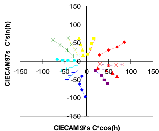
Figure 2. Hung and Berns (1995) lines of constant perceived hue in the CIECAM97s color space.
