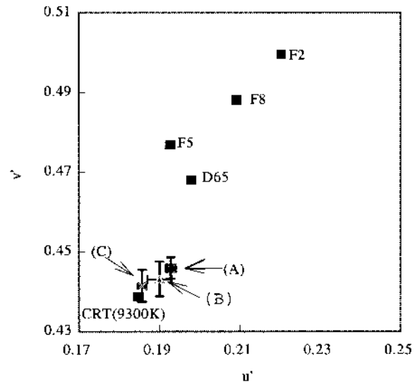
Figure 3. Shifts of adaptation points according to the chromaticities of illuminants.
