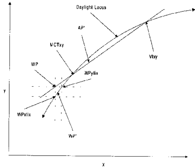
Figure 5. Calculation of new monitor white point (WP') for ICC profile format.
