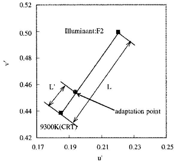
Figure 1. Calculation of shift ratio( L'/L ) in u' - v' coordinates.
