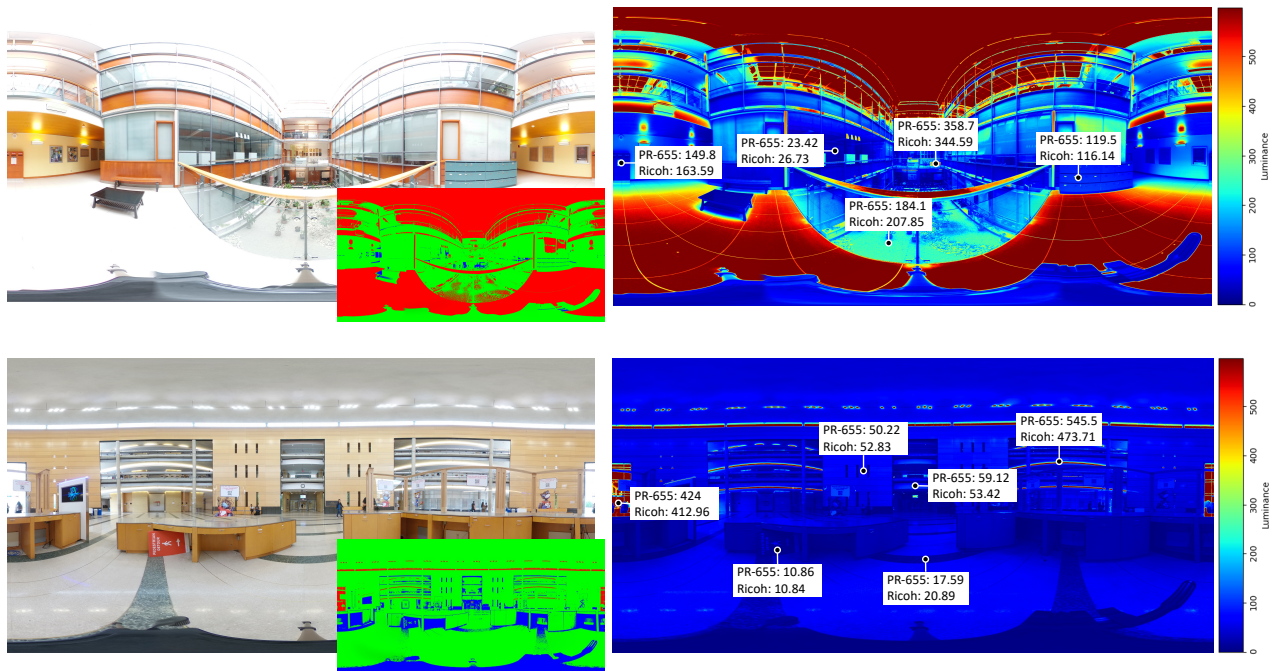
Figure 4. Luminance maps computed for two scenes. Shown is the JPEG image for the EV0 image which has been mapped to its rectilinear format. While the processed JPEG image appears bright, these scenes were relatively low-light as evident by the low luminance values. The inset shows the HDR composite map, where green is EV0, red is EV-1, and blue is EV+1. The corresponding luminance map is also shown. Readings using the SpectraScan PR-655 spot luminance meter were taken for reference against our results (see Results for description of the slight discrepancies between measurements).
