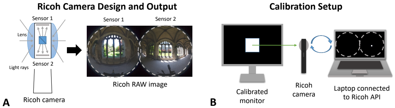
Figure 2. (A) An illustration of the Ricoh Theta Z1 device is shown. The optical paths of two fish-eye lenses are directed to two separate sensors. The camera is capable of outputting a single RAW image in which the two sensor images are concatenated side by side. (B) A calibration procedure is used to map the sensor intensities to luminance values. A calibrated LCD monitor displays images with specified luminance values, which are imaged by the Ricoh camera using varying ISO and shutter speeds.
