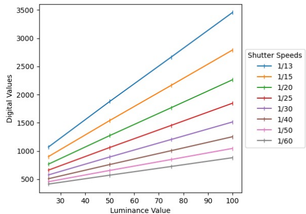
Figure 3. The RAW image’s response (digital values) with respect to the luminance for different shutter speeds. This plot is for ISO 80, the default ISO of the camera. The sensor responds linearly to incoming scene luminance.
