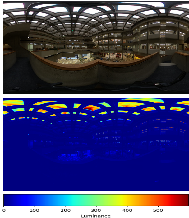
Figure 1. (Top) The output of a single omnidirectional 360° JPEG image from a Ricoh Theta Z1 camera. (Bot) The corresponding omnidirectional luminance map computed from calibrated RAW images using multi-exposure fusion.
