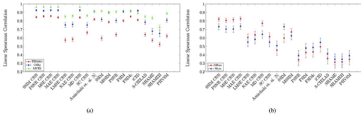
Figure 3. Spearman correlation values the enhanced CNN based IQMs along with other state-of-the-art IQMs calculated for the (a) TID2013, CSIQ, and LIVE2 datasets and (b) CDLIQ dataset viewed at a distance of 50 and 100 cm shown with 95% confidence intervals.
